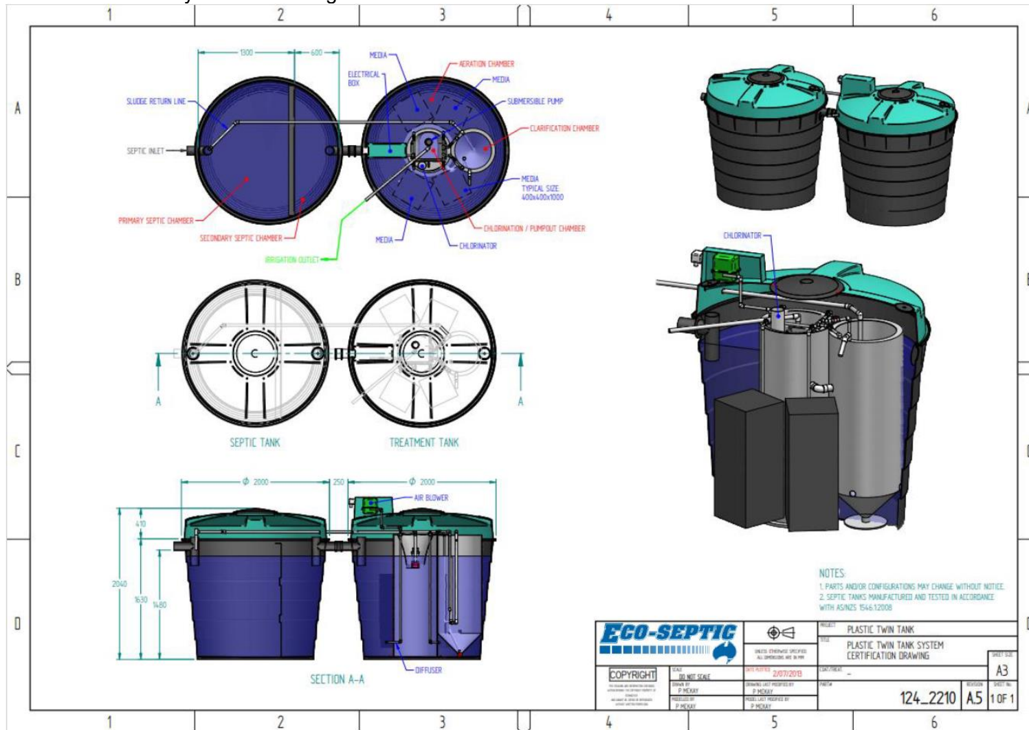
Attachment 3 – Eco Pro Twin Poly Schematic diagram
