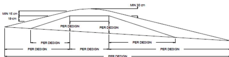
FIGURE 10: CROSS SECTION – MOUND SYSTEM
