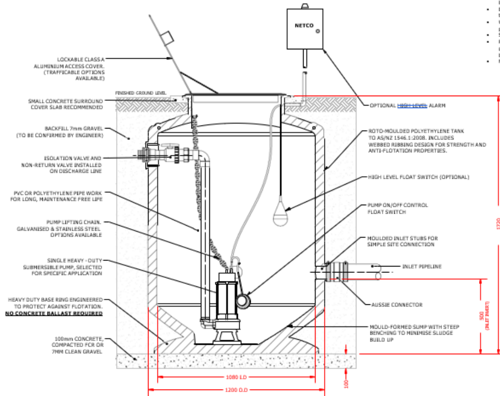
PUMP STATION TYPICAL SECTION
